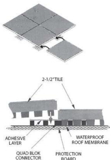
1. Typical Tile Field Placement
