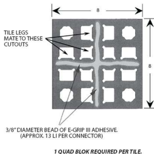
2. Connector Detail
